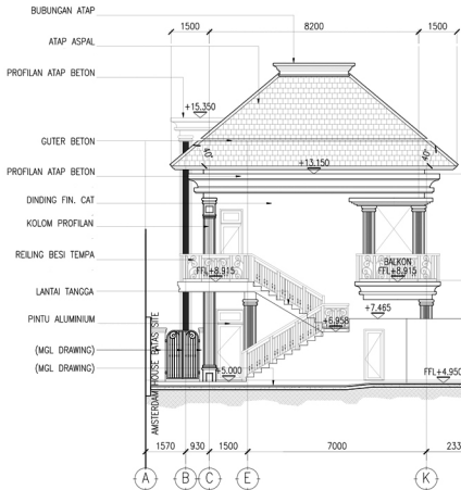
1 A2-101 MANADO AMSTERDAM HOUSE TAMPAK A SCALE 1 : 150
